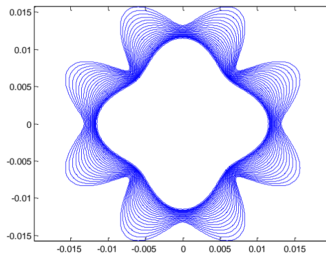
Figure6 , Time evolution of Newtonian fluid in the circular cell
