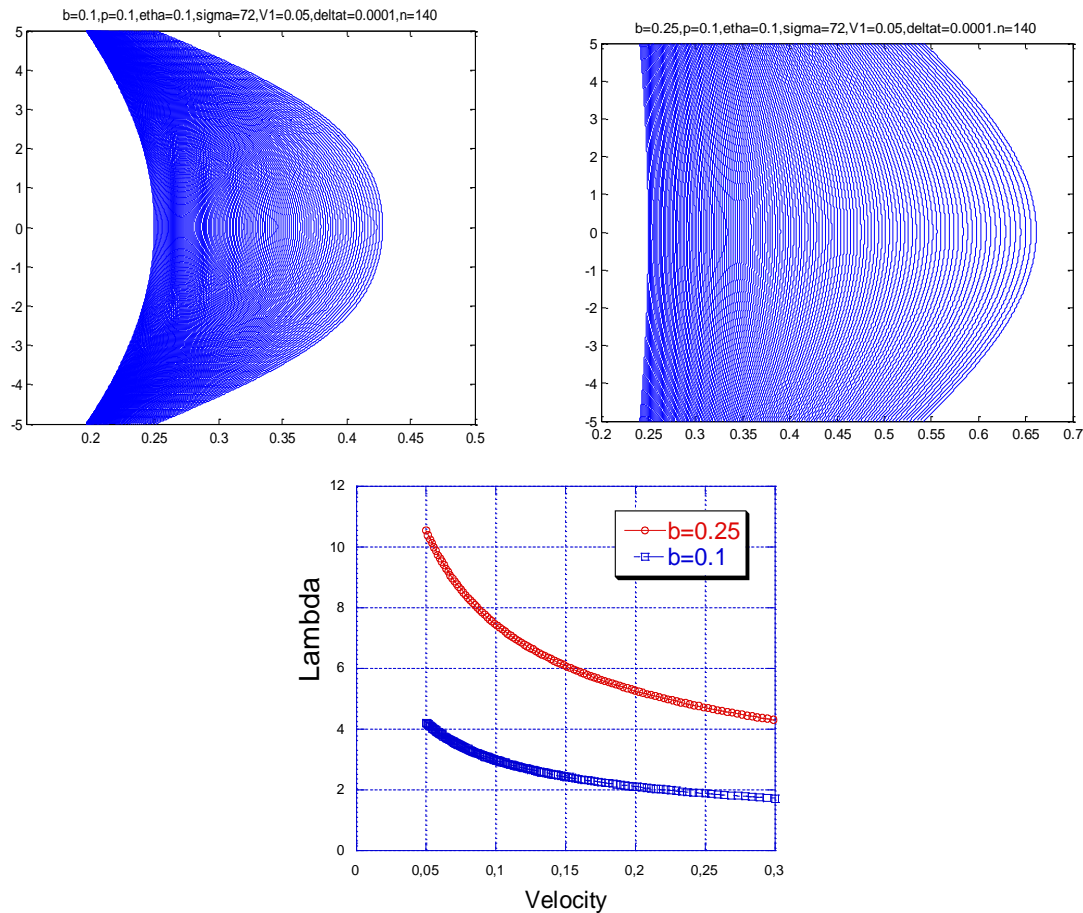
Figure3 , output of program for (a) b=0.25 and (b) b=0.1 , (c) comparison of wave-lengths graph
