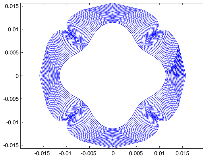
Figure 8 , Time evolution of a non-Newtonian fluid in the circular cell based on Kondic's model
