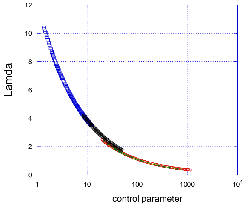
Figure5 , wave-length graph unit age control parameter
