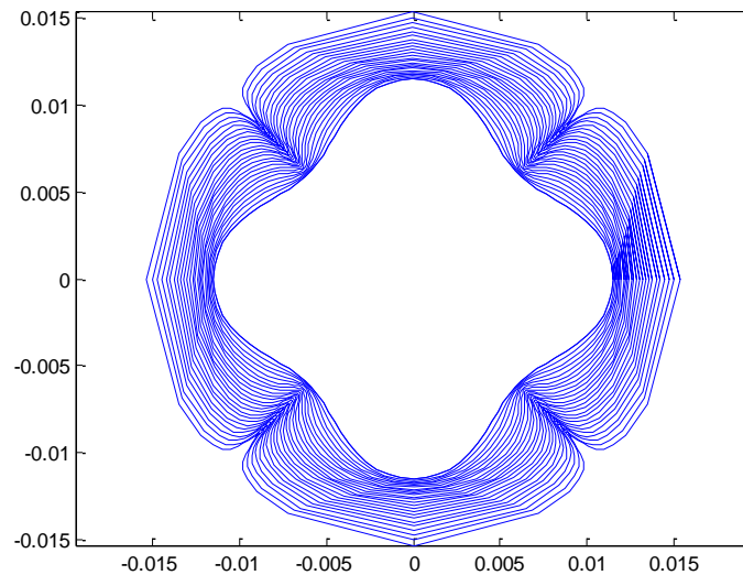
Figure 7 , Time evolution of a non-Newtonian fluid in the circular cell based on Bonn's model
