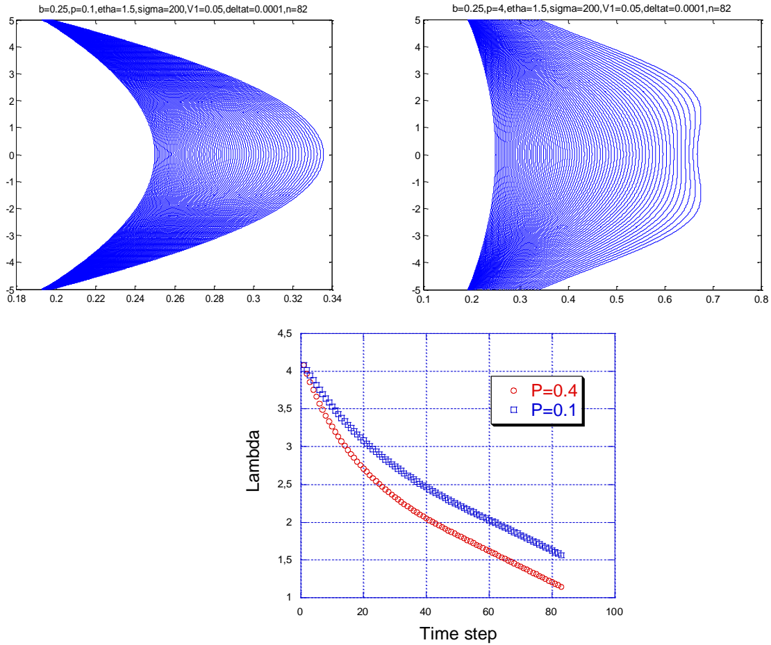
Figure4 , Exercised pressure is in a) 0.1 and b) 0.4. Graph c) shows the fluid in more pressure perturbs rather and forms finger
